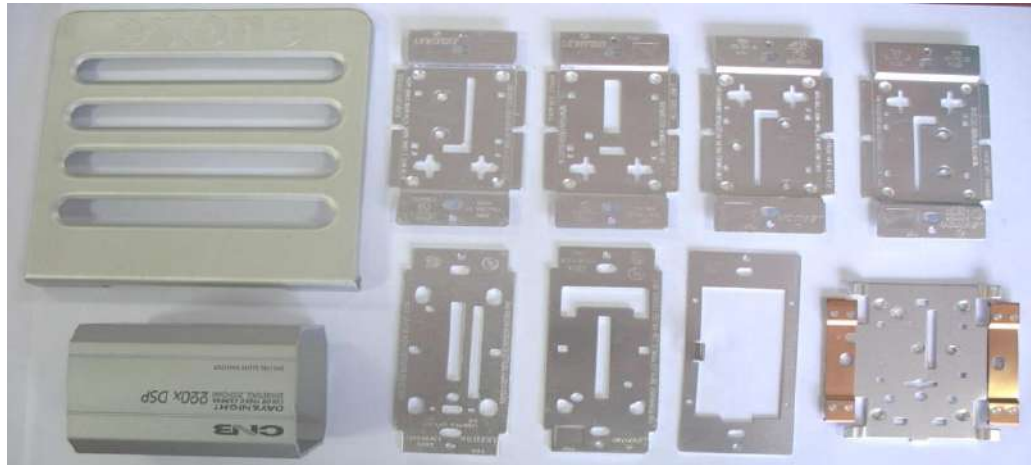
Panel Stand
